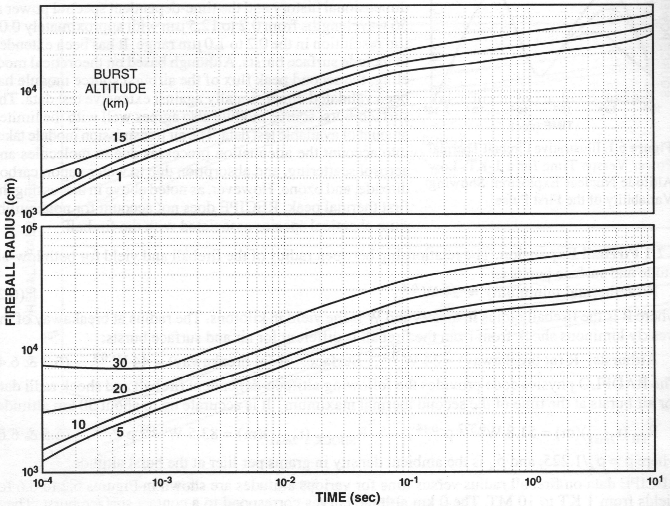
Figure 6.3. Fireball Radius Versus Time Curves for a 10-KT Burst at Various Altitudes.
